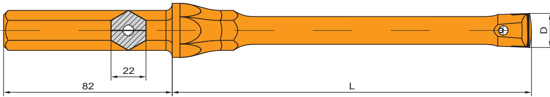
Plug hole integral steel Hex 22 x 82 mm
