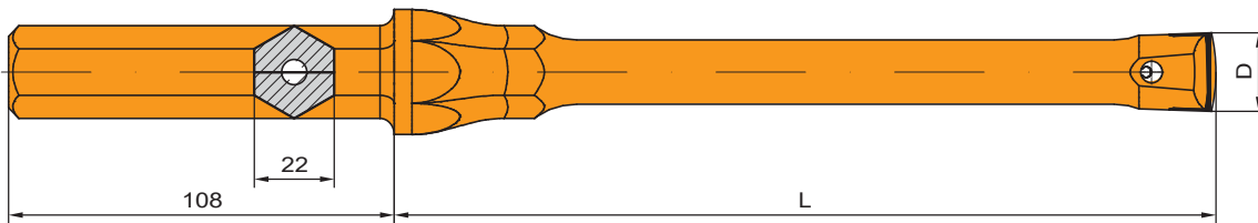
Plug hole integral steel Hex 22 x 108 mm
