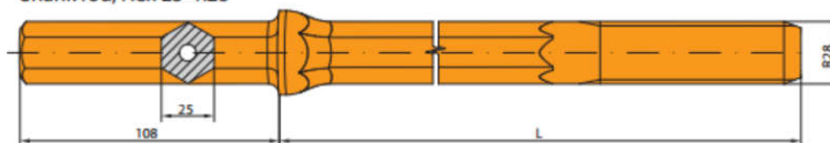
Shank rod, Hex 25- R28
