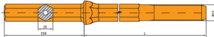
Shank rod, Hex 25 - R25
