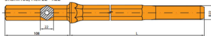
Shank rod, Hex 22 - R22
