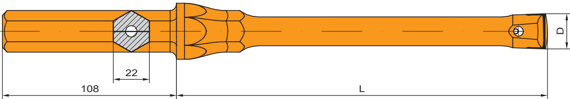
Plug hole integral steel Hex 22 x 108 mm
