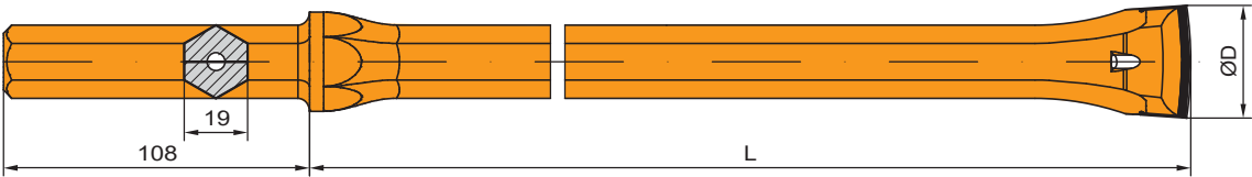
Shank Hex 19 x 108 mm
