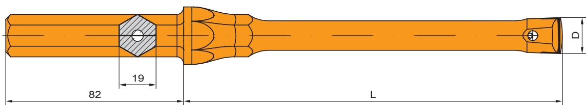
Plug hole integral steel Hex 19 x 82 mm
