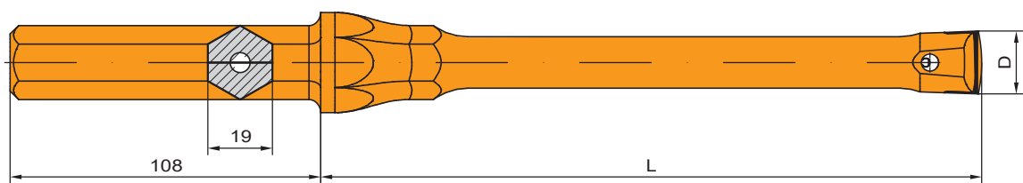
Plug hole integral steel Hex 19 x 108 mm
