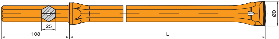
Shank Hex 25 x 108 mm
