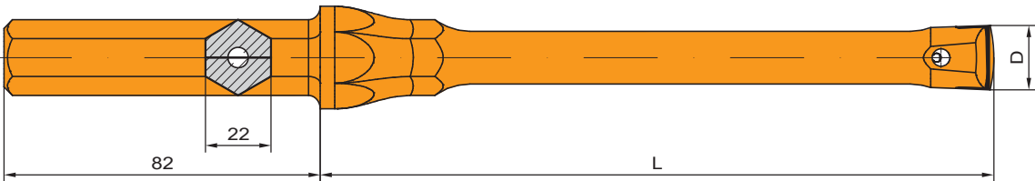
Plug hole integral steel Hex 22 x 82 mm
