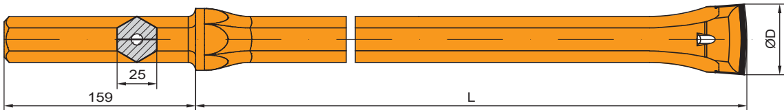
Shank Hex 25 x 159 mm
