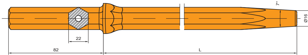
Tapered rod, shank Hex 22 x 82 mm
