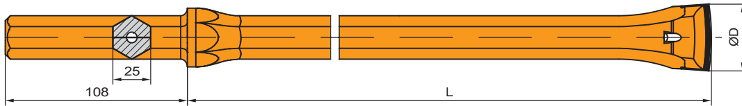
Shank Hex 25 x 108 mm
