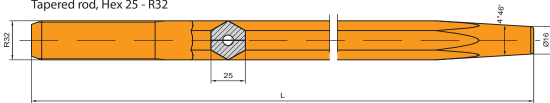
Tapered rod, Hex 25 - R32
