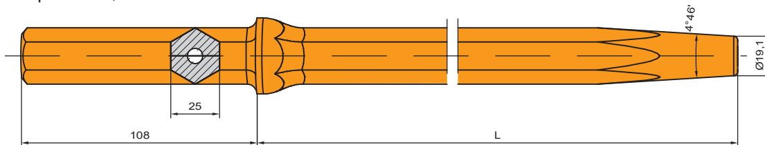
Tapered rod, shank Hex 25 x 108 mm
