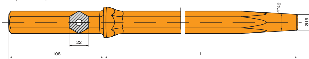
Tapered rod, shank Hex 22 x 108 mm
