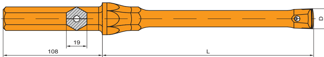
Plug hole integral steel Hex 19 x 108 mm
