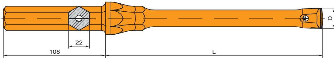
Plug hole integral steel Hex 22 x 108 mm
