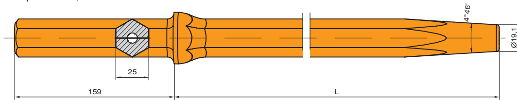
Tapered rod, shank Hex 25 x 159 mm
