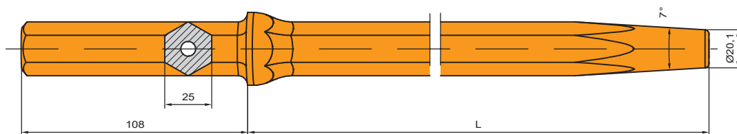
Tapered rod, shank Hex 25 x 108 mm
