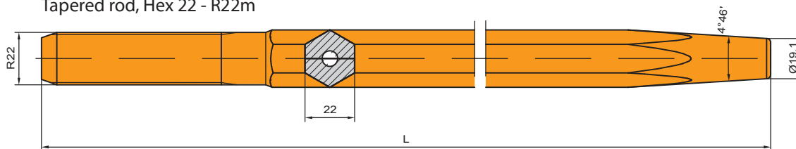
Tapered rod, Hex 22 - R22m
