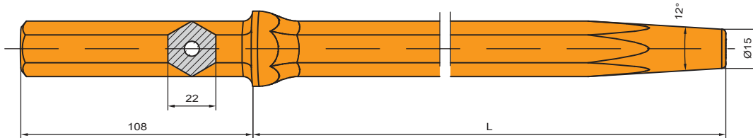
Tapered rod, shank Hex 22 x 108 mm
