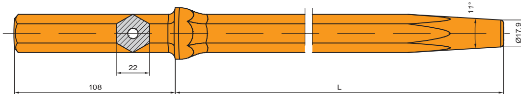
Tapered rod, shank Hex 22 x 108 mm
