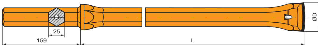
Shank Hex 25 x 159 mm
